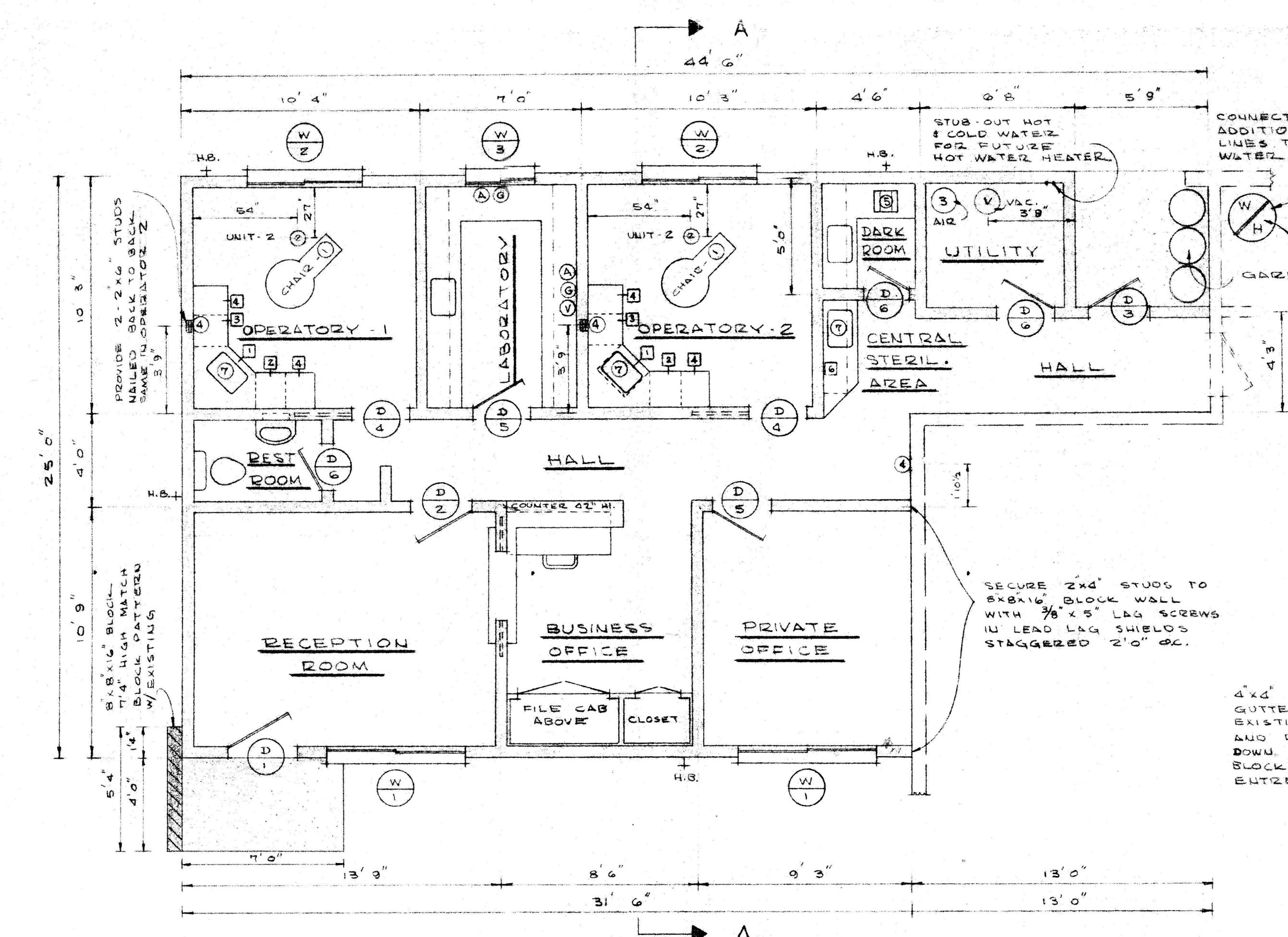
FLOOR PLAN
